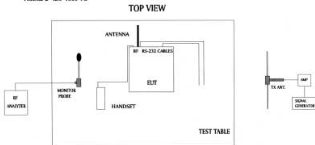
FIGURE 2 - IEC 1000-4-3
