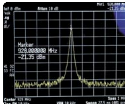
Dragon output on a spectrum analyzer.
