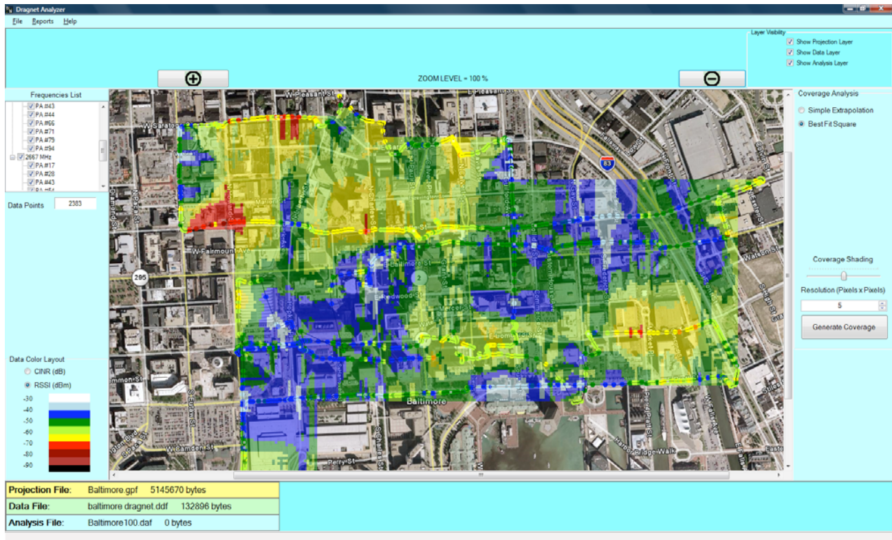
Figure 1 – Dragnet Analyzer
