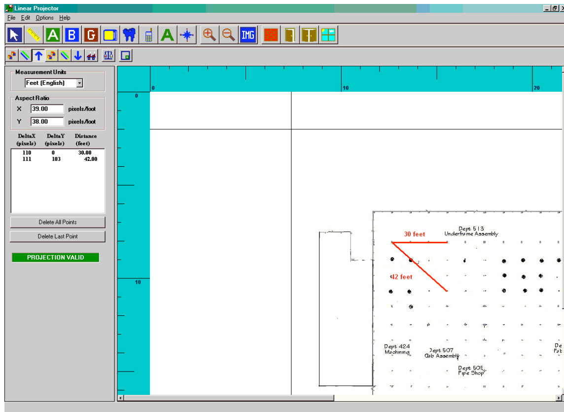
Figure 2 – Quick Projection
