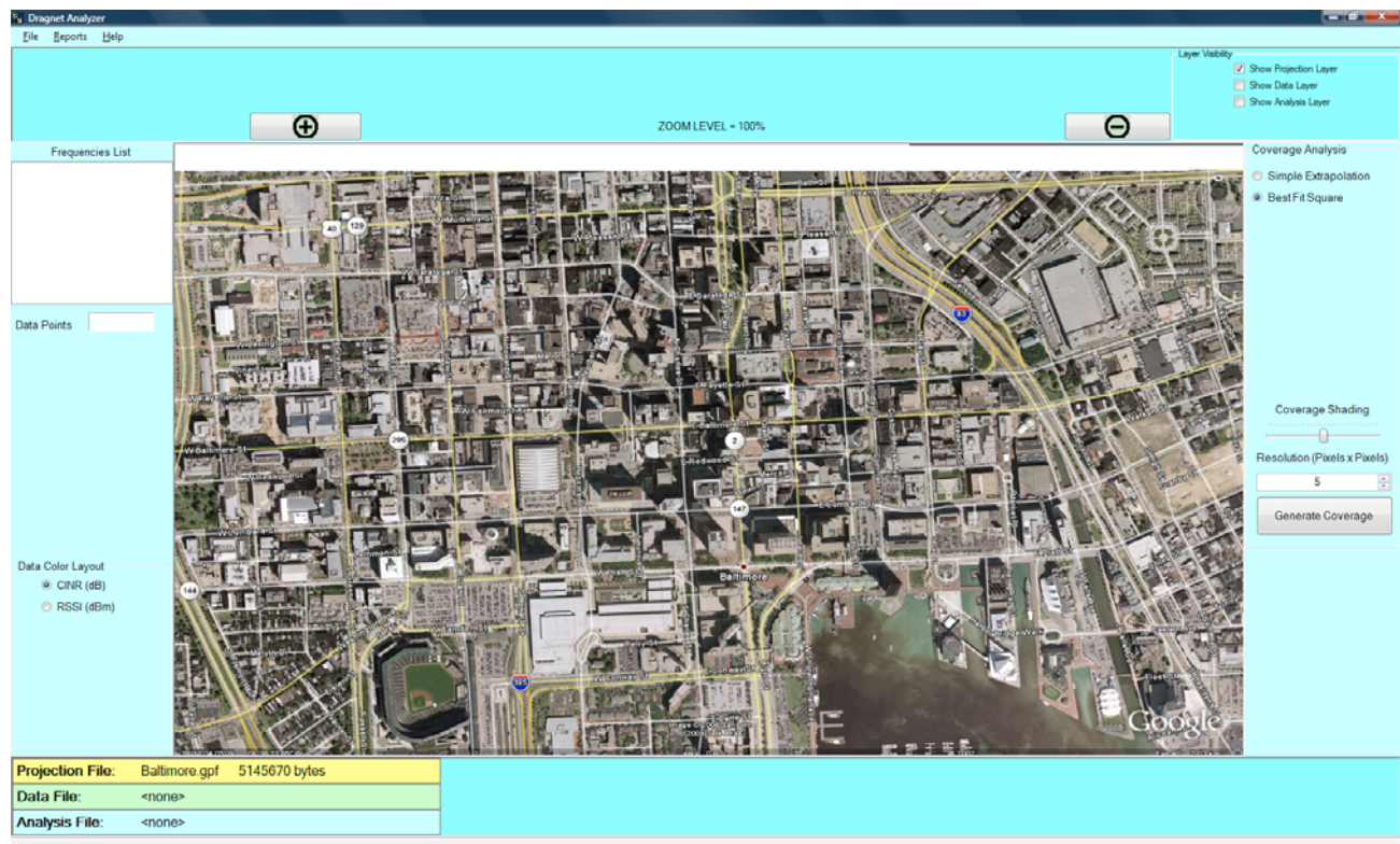
FIGURE 2 – Projection Layer
