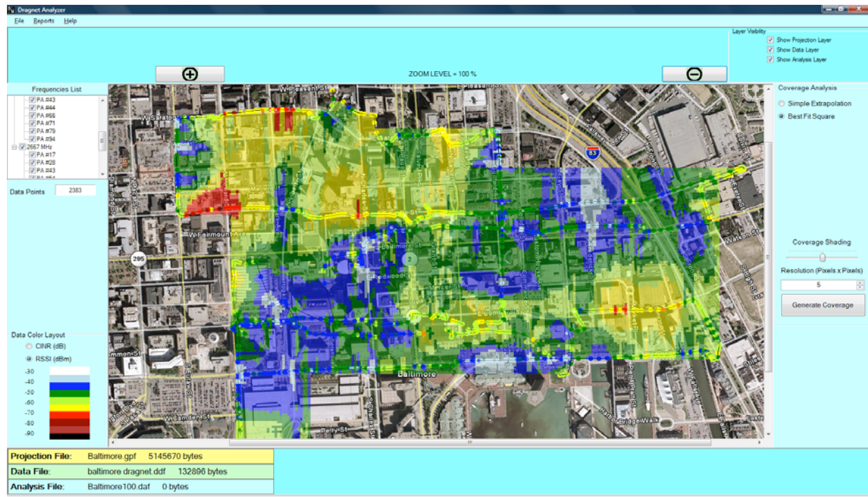
FIGURE 6 – Best Square
