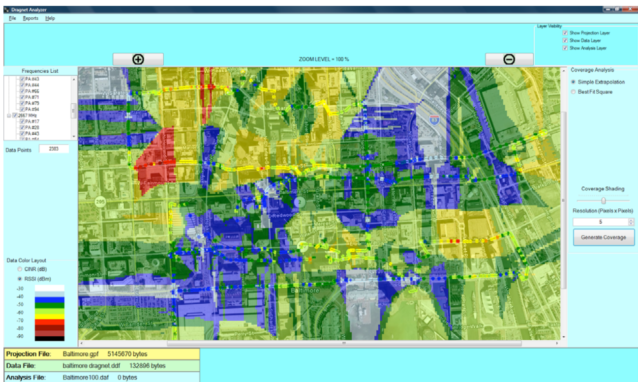
FIGURE 5 – Simple Extrapolation
