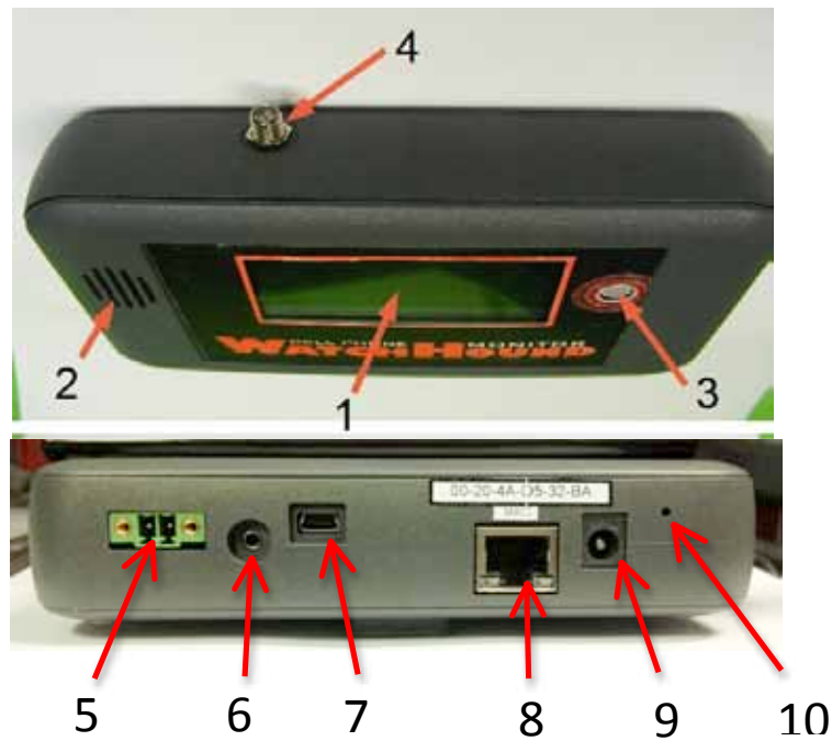
Figure 3. Watchhound Unit User and Electrical Interfaces
